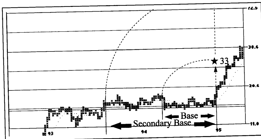
Figure 11.20 A one box reversal point and figure chart of Intel using percentages. A reversal of 3.2% is needed to move into the next column. Measuring horizontally from right to left along the base, upside counts can be made to 33 and then to 87.6 (see arcs). (Chart courtesy of UST Securities Corp.)
