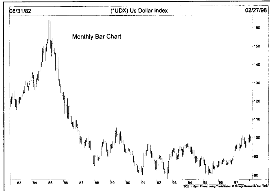
Figure 3.10 A monthly bar chart of the U.S. Dollar Index. Each bar represents one month's price data. By compressing the data even further, the monthly chart allows chart analysis for periods as long as twenty years.
