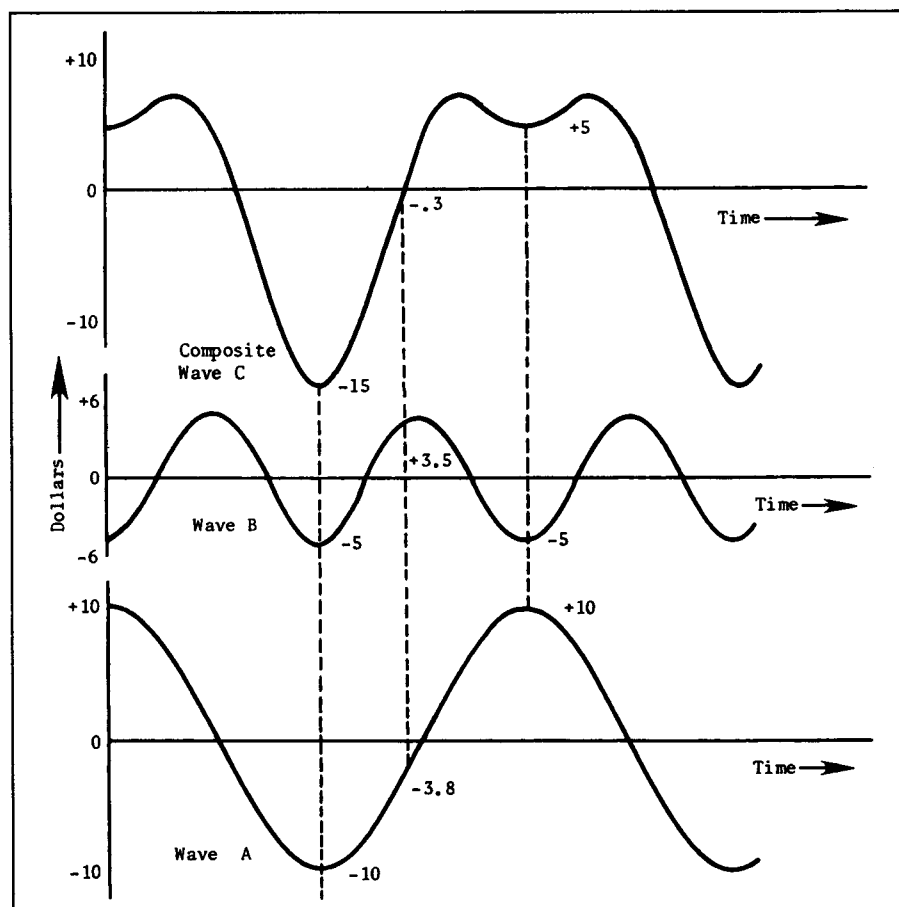
Figure 14.8 The summation of two waves. The dotted lines show how, at each point in time, the value of wave A is added to the value of wave B to produce the value of composite wave C.
